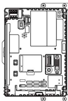
Standard installation (portrait)
