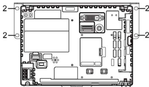
Standard installation
