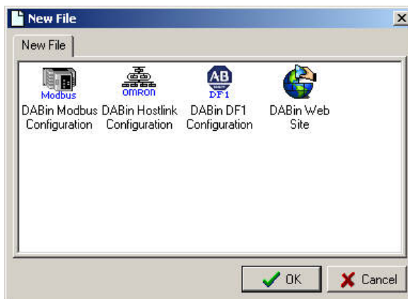
Figure 44 - New File dialog box
