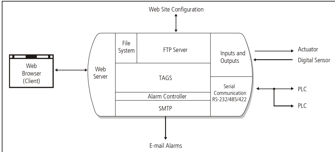
Figure 1 - DABin functional diagram
