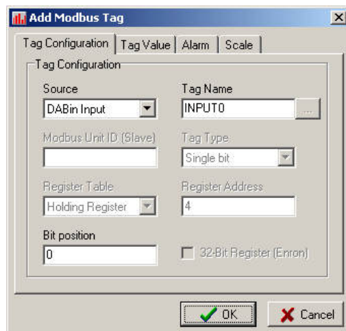
Figure 33 - Digital Inputs / Output Tag Configuration
