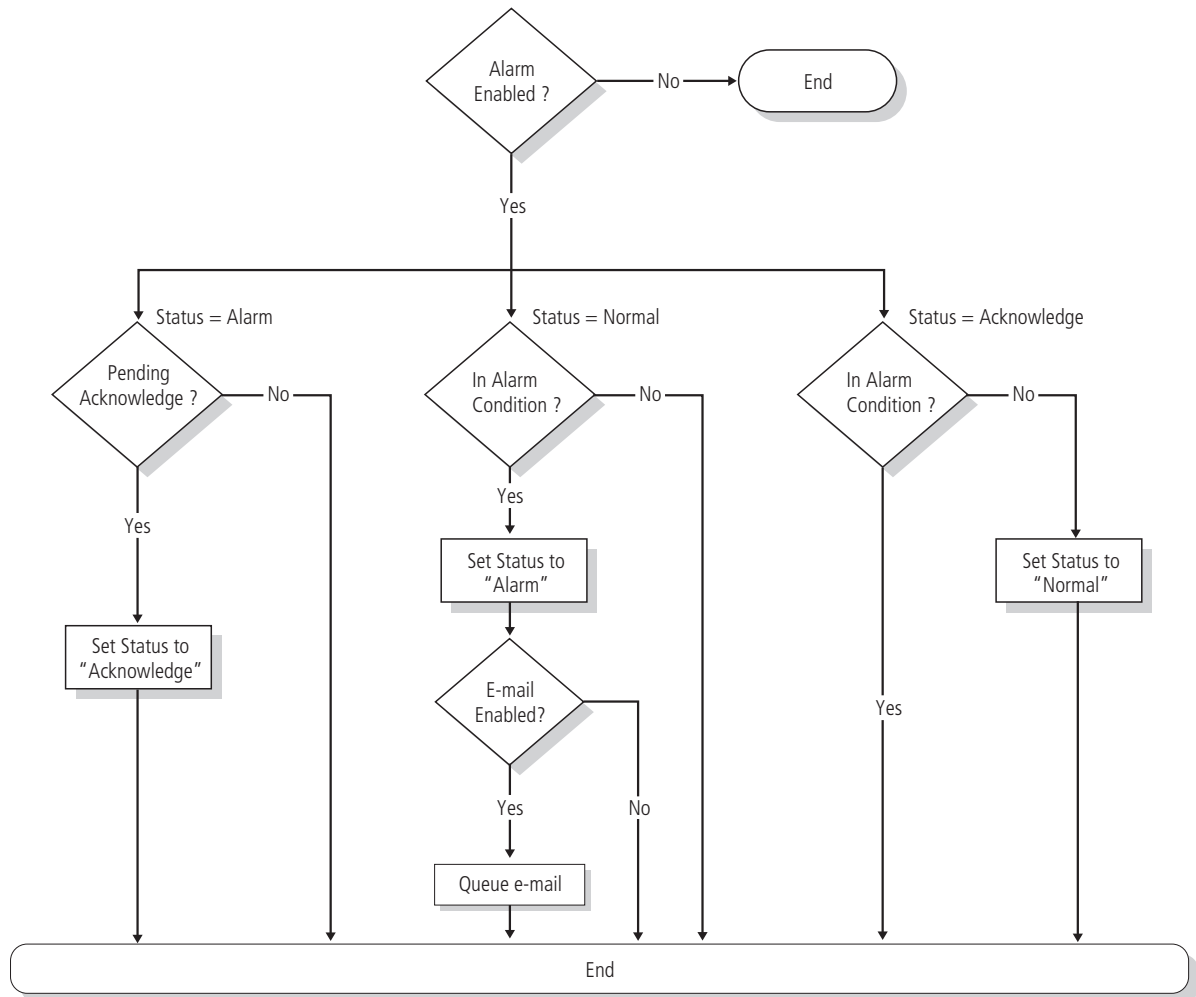
Figure 60 - Alarm Control Cycle of DABin DF1
