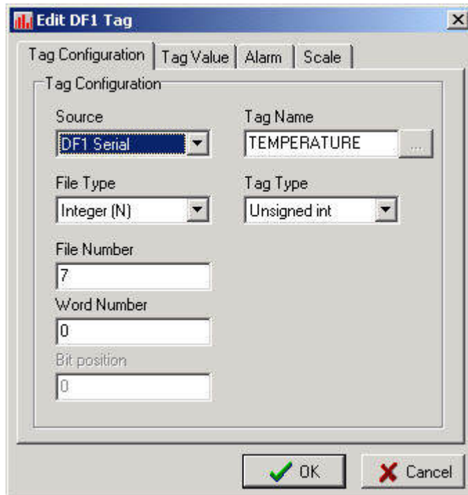
Figure 66 - DF1 Tag Configuration
