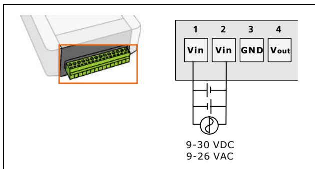
Figure 3 - Power connection detail
