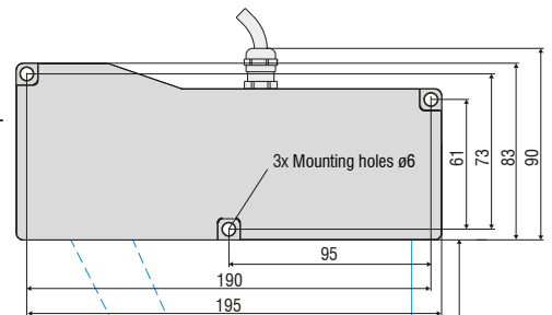
optoNCDT 2300-2BL / 2300-5BL / 2300-10BL Direct reflection
