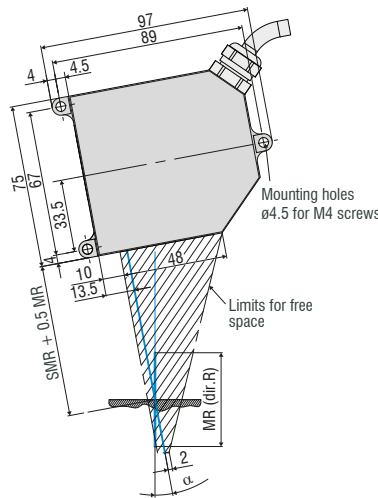
optoNCDT 2300-2BL / 2300-5BL / 2300-10BL Direct reflection
