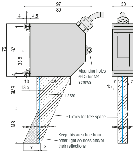
optoNCDT 2300-2BL / 2300-5BL / 2300-10BL Diffuse reflection
