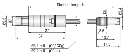
Sensor cable with connector type C
