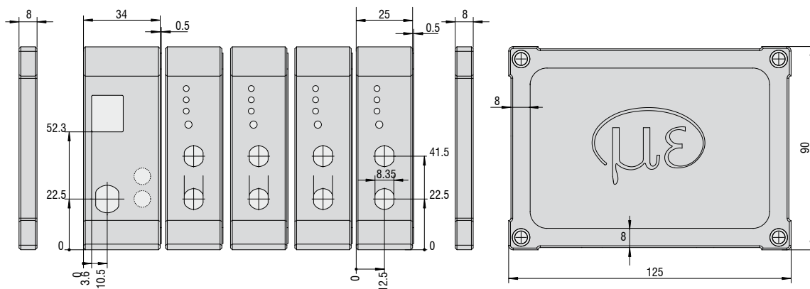
Controller DT6222 Demodulator DL6222 DL6222 DL6222
