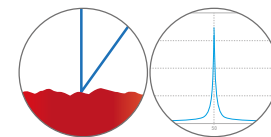
Positioning a welding head in automated welding units: no influence by red radiation
