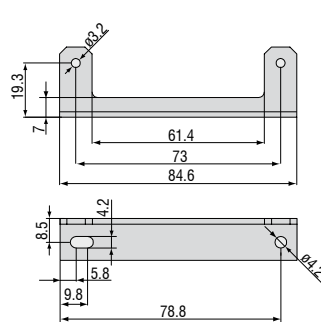
Mounting adapter CP6001
