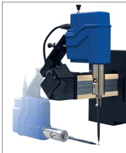
fully automated arm orientation mechanism
